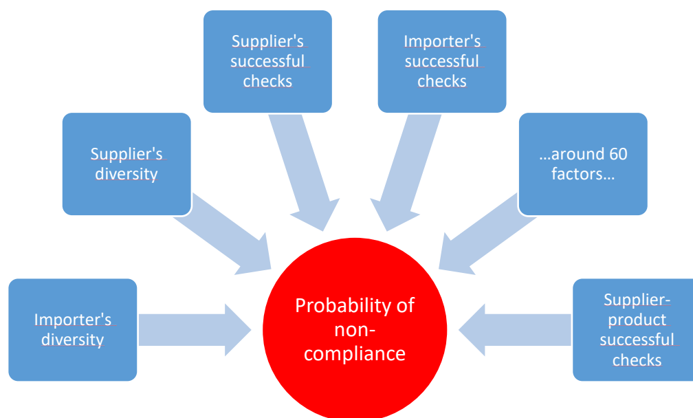
Figure 9. Probability factors
